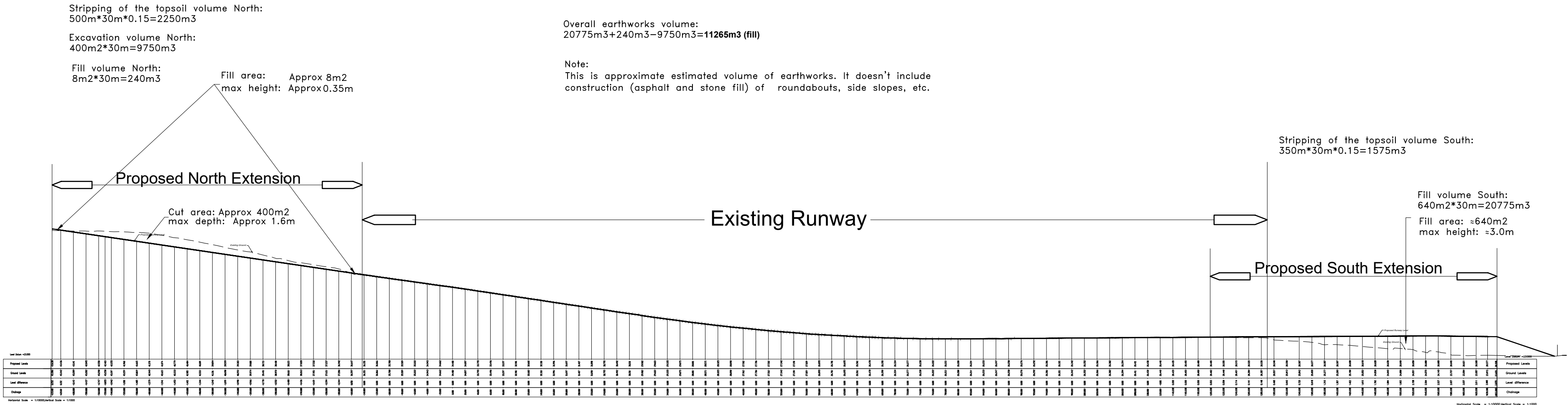
RUNWAY LONGITUDINAL SECTION
